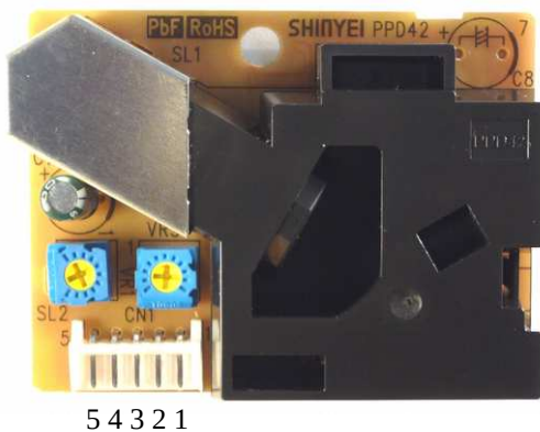
Figure 6 - PPD42 particle sensor with connector pin numbering shown
