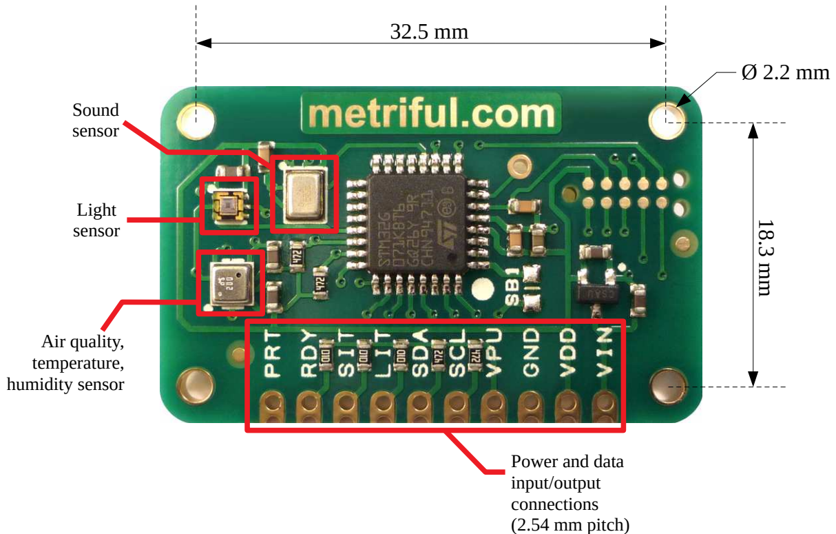
Figure 1 - Position of sensors and mounting holes on the MS430 circuit board.
